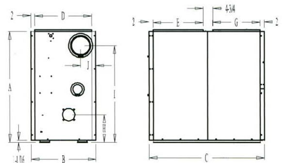
LO Series
